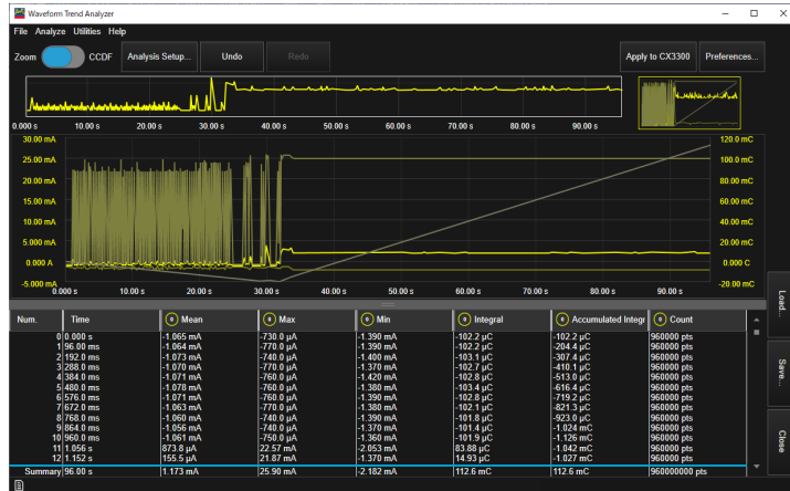
Figure 18. Waveform trend
