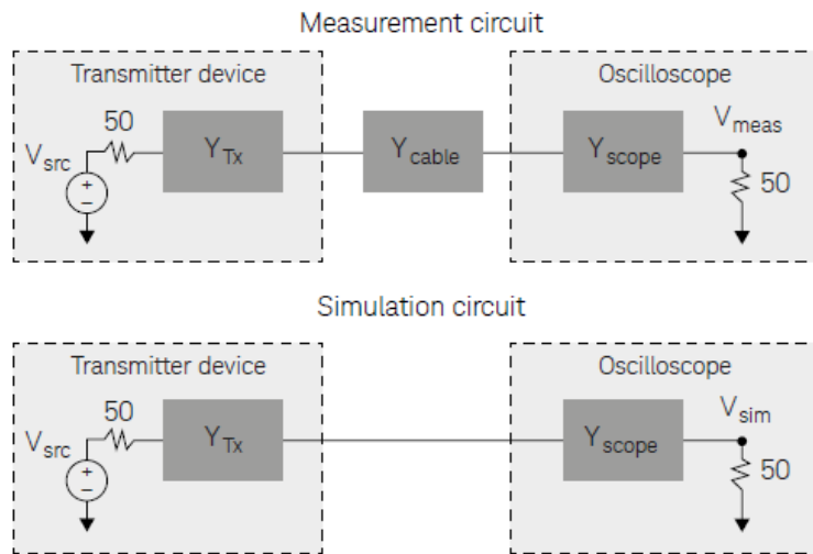
Figure 15. InfiniiSim handles the removal of the cable effects
