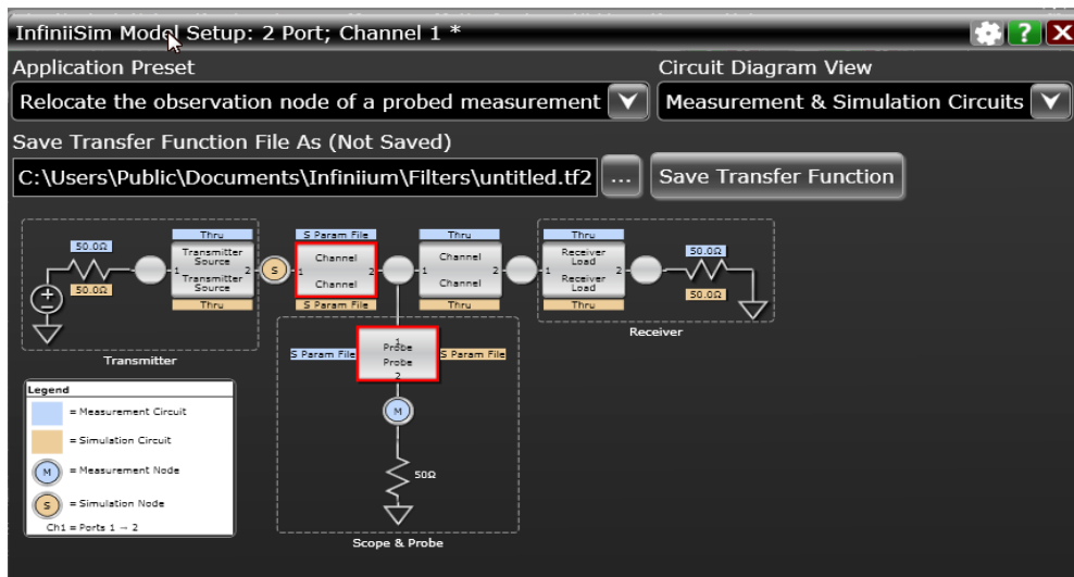
Figure 20. Measurement and Simulation circuits. Blue designates the measurement circuit elements while the brown labeling designates the simulation circuit elements.
