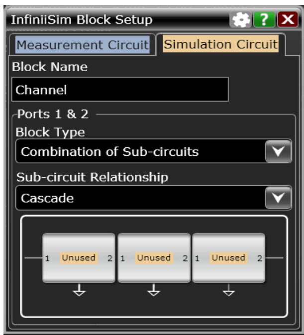
Figure 19. Sub-circuit capability: Any given InfiniiSim standard block can be described as a combination of sub-circuits.
