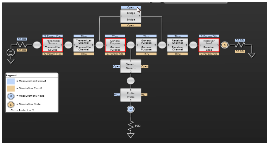
Figure 18. InfiniiSim can handle the most sophisticated system configurations with general-purpose 9- block configuration shown above
