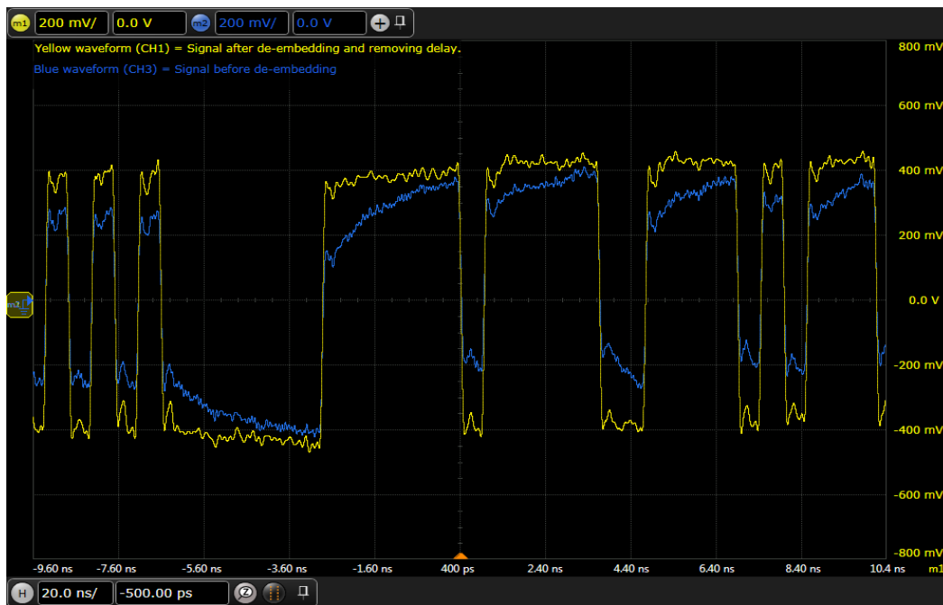
Figure 21. De-embedded, yellow, channel 1 waveform along with original channel 3 waveform.
