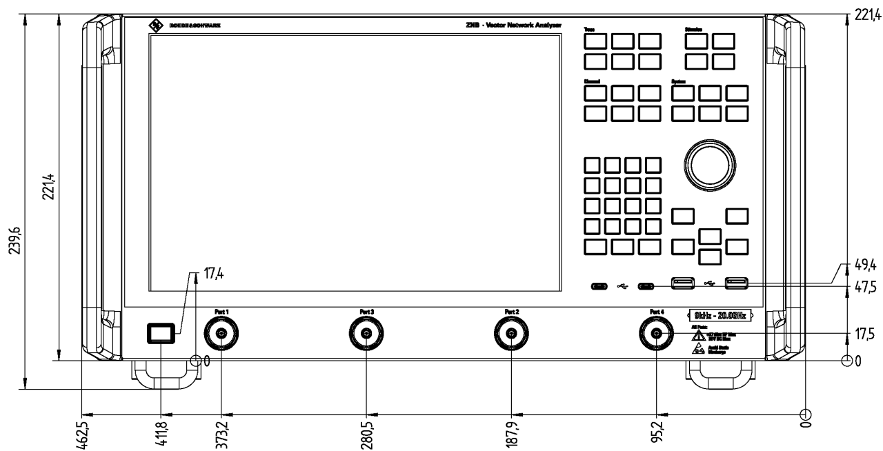
Front view of the R&S®ZNB3000
