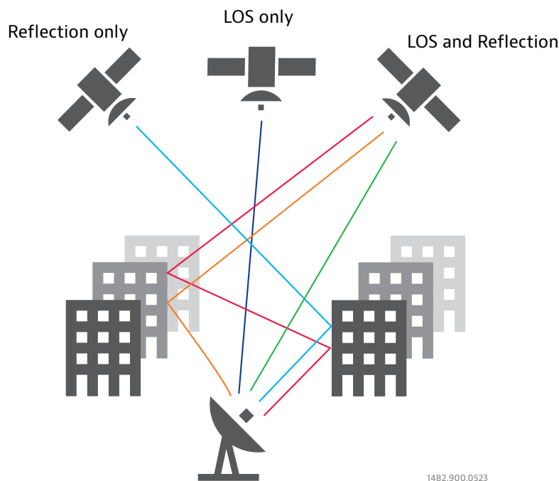
GPS Antenna Placement for Data Center Applications
