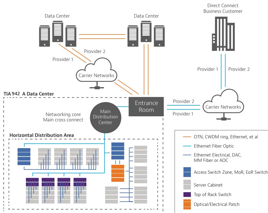
Typical Data Center Internal and External Connectivity
