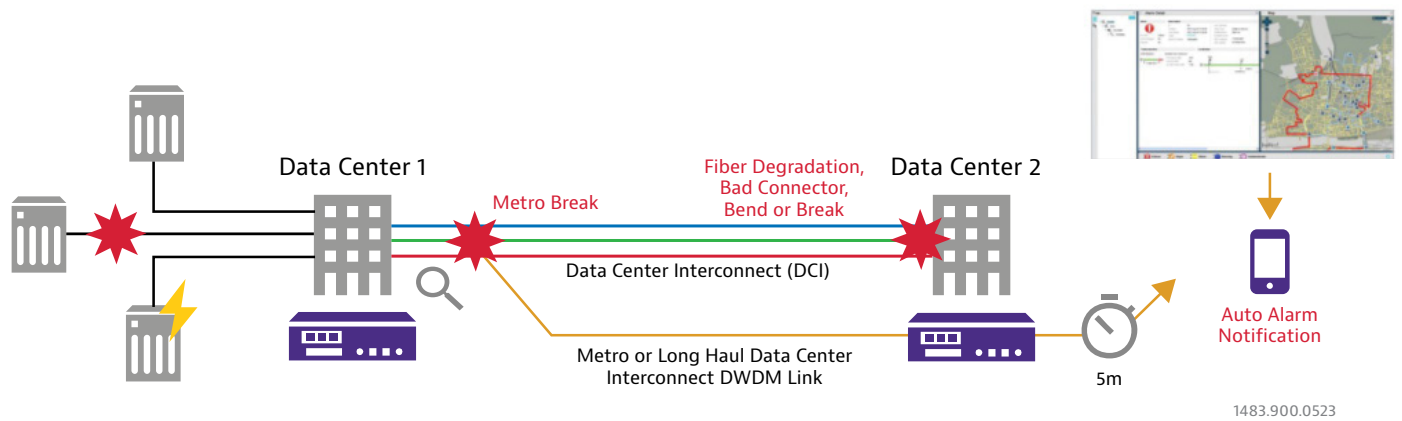
Auto Detect Vulnerabilities in a Data Center Network
