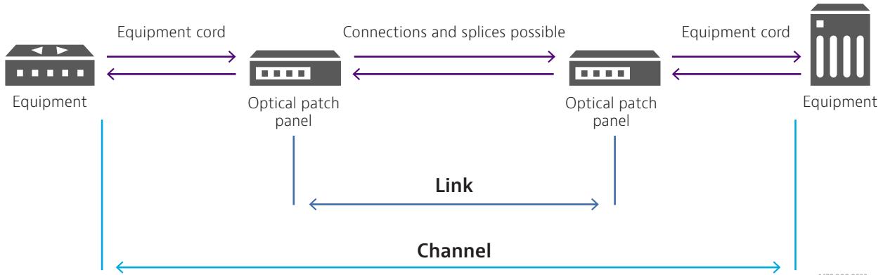
Typical Data Center Physical Cabling Infrastructure
