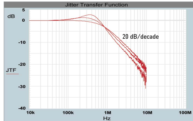
Figure 27. Three selectable frequency response settings. The example shows JTF loop bandwidth of 900 kHz and 0 dB, 1.2 dB, 2.8 dB peaking
