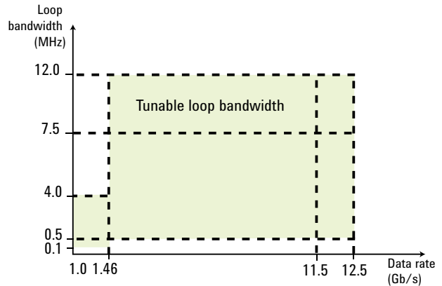
Figure 26. CDR loop bandwidth
