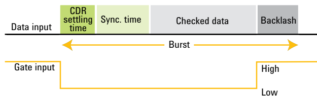
Figure 28. Burst mode allows recirculation loop testing
