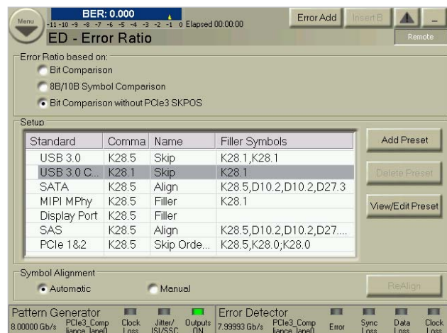
Figure 29. SER analysis option enables receiver tolerance testing of devices using retimed, coded loopback.
