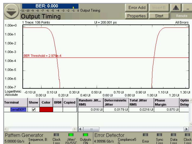
Figure 9. BERT scan including RJ/DJ separation, total jitter
