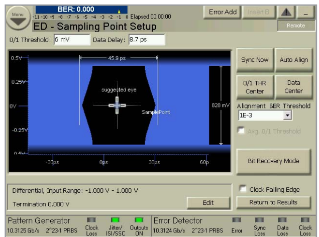
Figure 11. Auto alignment (center) simplifies correct sampling
