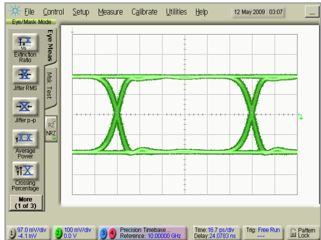
Figure 15. Clean output signal; 10 Gb/s, 400 mV amplitude
