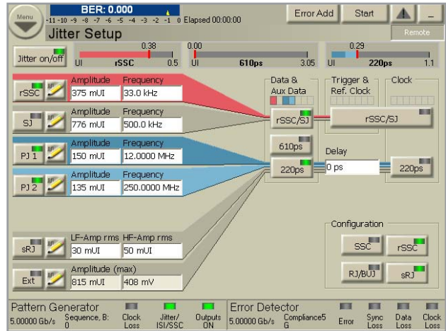
Figure 3. Manual jitter composition. This allows a combination of jitter types to be injected. Example shows a typical jitter setup for a PCIe 2.0 add-in card test
