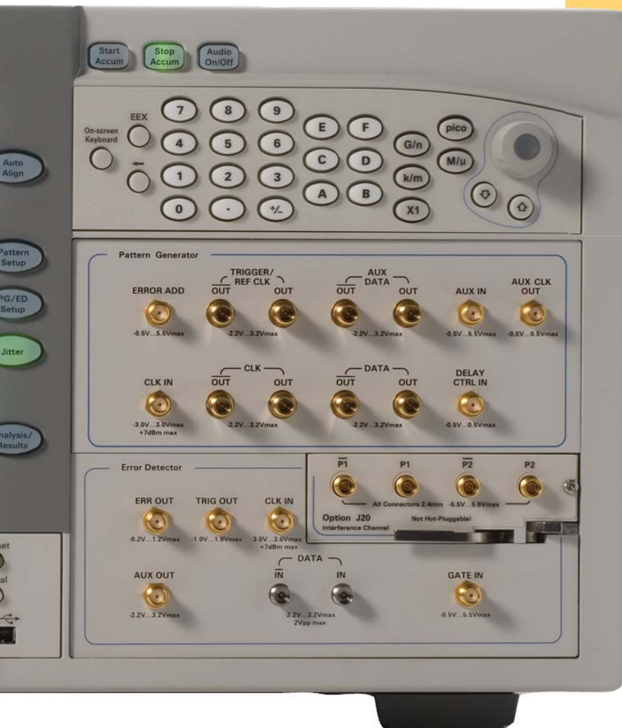
Figure 2. J-BERT N4903B The most complete jitter tolerance test solution for testing embedded and forwarded clock devices
