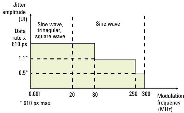
Figure 18. Periodic jitter maximum for data rates ≤ 3.375 Gb/s using the 610 ps delay line
