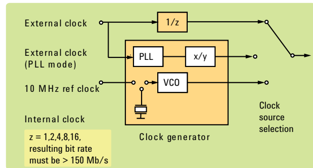
Figure 16. N4903B supports multiple clock modes
