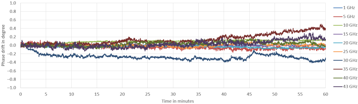
Measured phase drift between RF inputs versus time for different RF frequencies
