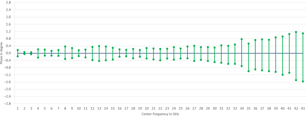
Measured retune phase repeatability, preamplifier off, minimum and maximum value after 100 center frequency changes, referenced to average
