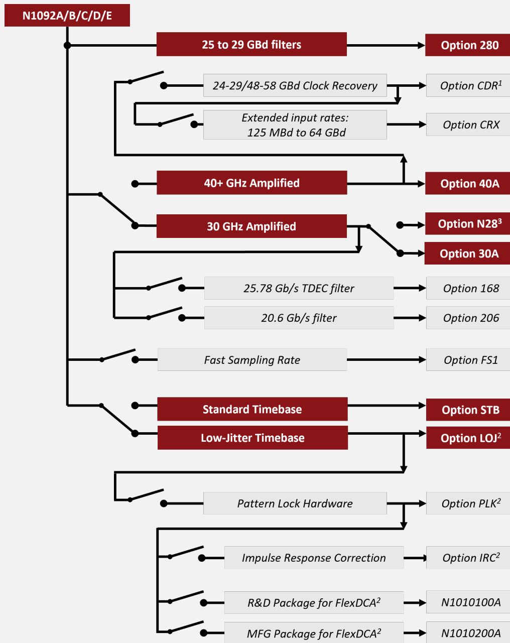
Figure 31. N1092A/B/C/D/E configuration chart
