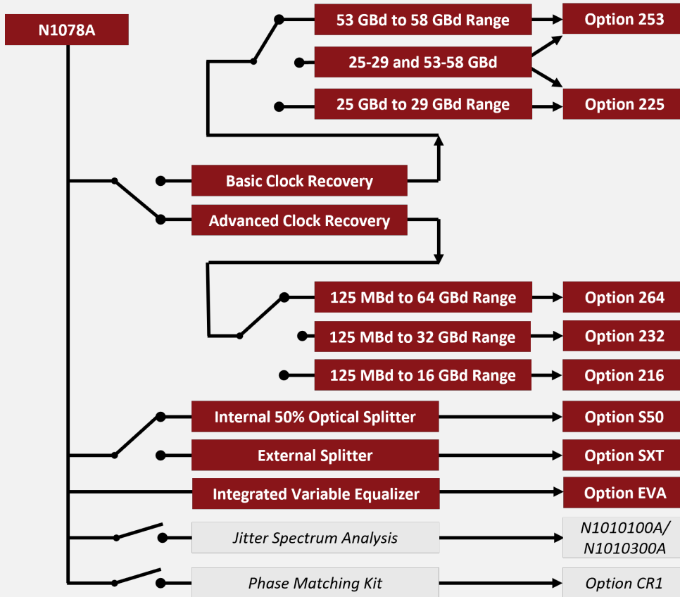
Figure 27. N1078A configuration chart
