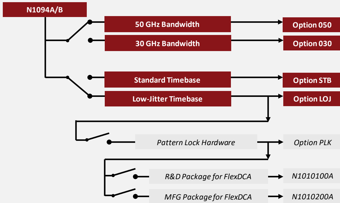
Figure 36. N1094A/B configuration chart
