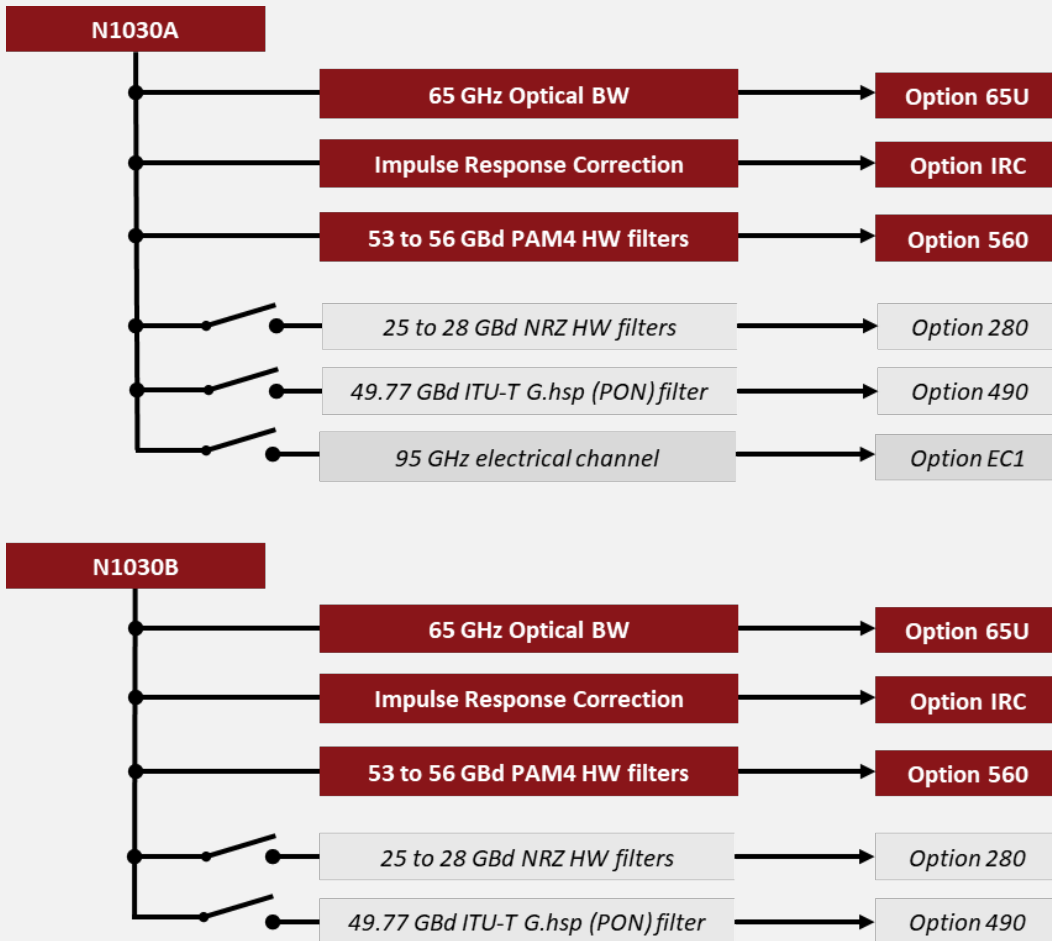
Figure 9. N1030A/B configuration chart
