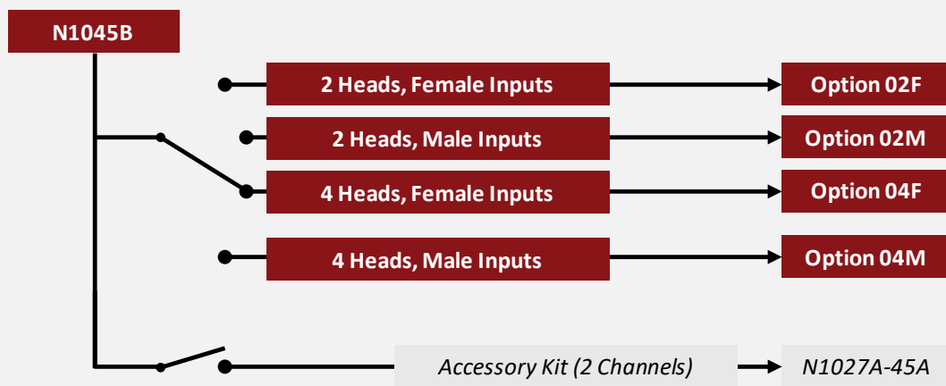
Figure 13. N1045B configuration chart
