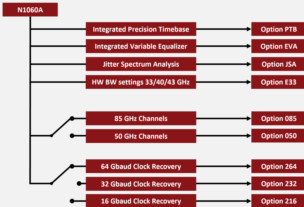
Figure 19. N1060A configuration chart
