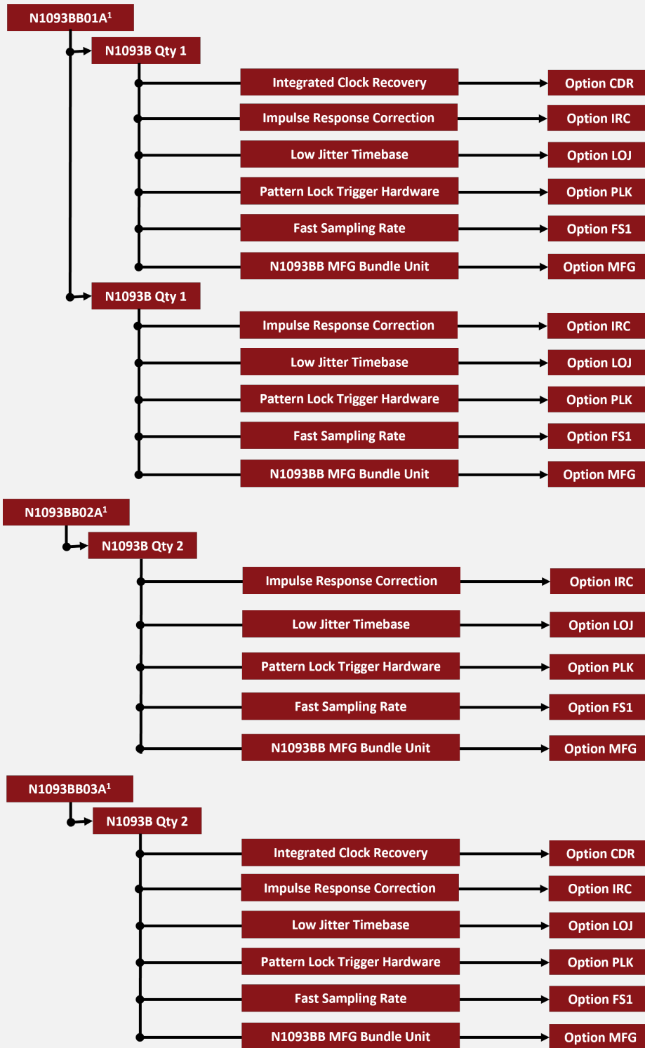
Figure 34. N1093BB0xA configuration chart
