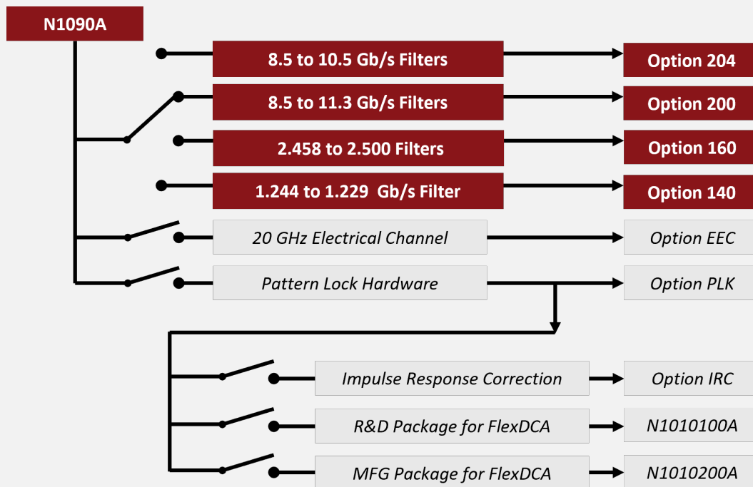
Figure 29. N1090A configuration chart
