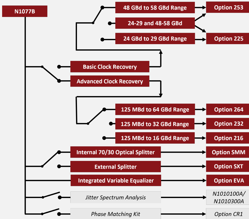
Figure 24. N1077B Multimode/Single-mode optical/electrical clock recovery with options 264 and SMM
