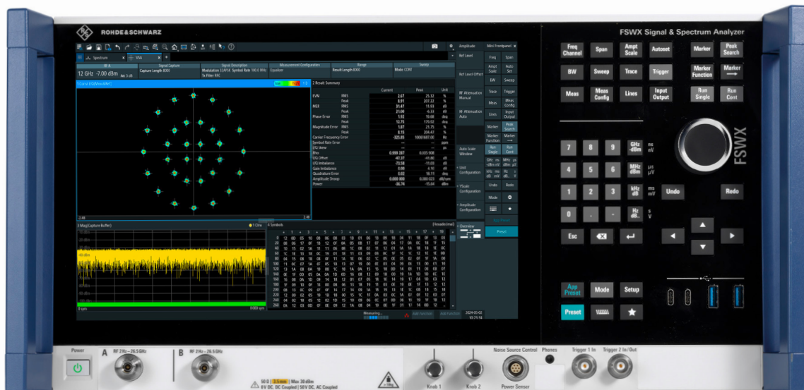
FSWX front view
