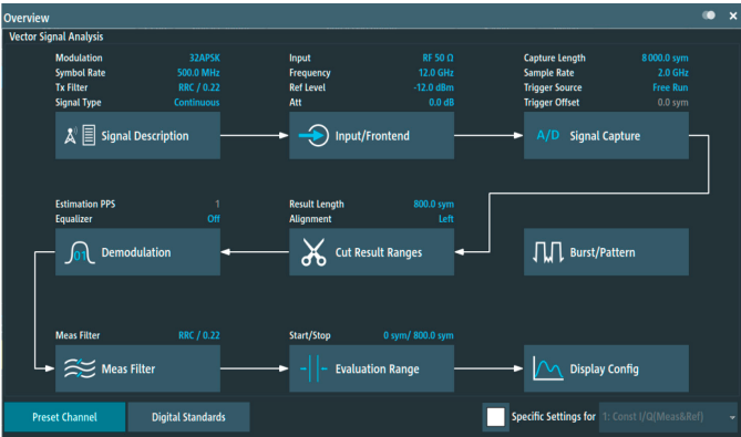
Clearly structured block diagram display
