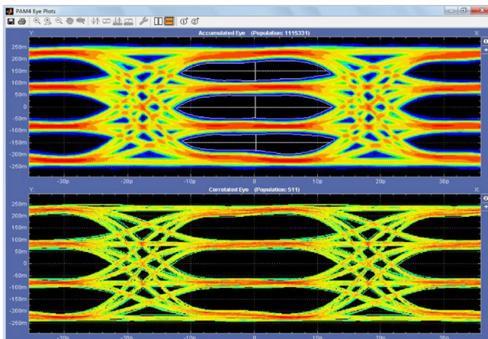
NRZ and PAM4 measurements - The throughput of Datacom networks continues to increase. Tek's MSO/DPO73304DX supports up to 10GBASE-KRn data rates. The powerful combination of the MSO/DPO7000DX and DPO7000SX Series oscilloscopes, DPOJET Jitter and Noise Analysis, PAMJET Signal Analysis, and the SDLA Serial Data Link Analysis tool performs accurate de-embedding and eye diagram analysis for Datacom standards.
