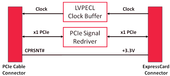
Figure 2. M9045B diagram
