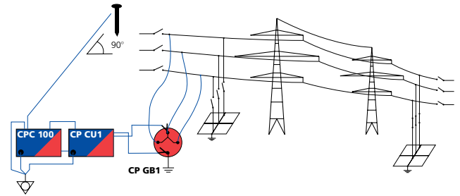
Ground Impedance Measurement
