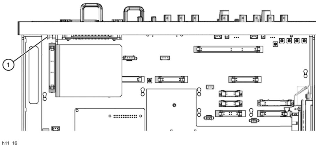
Figure 13 Hard Disk Drive Assembly Shield Reinstallation
