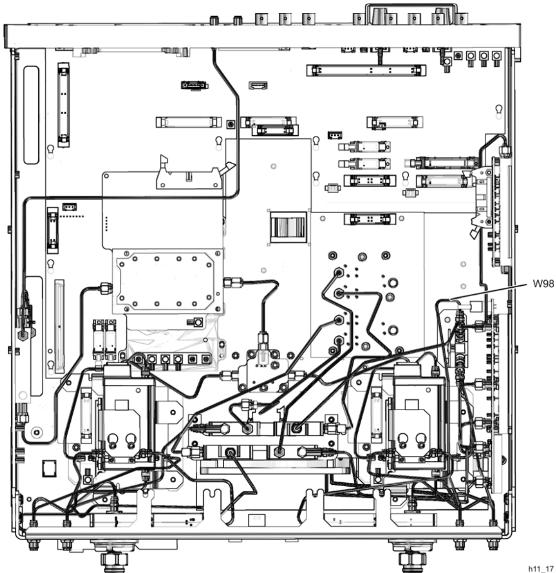
Figure 17 Switch Cable Replacement (E8361A/C Only)
