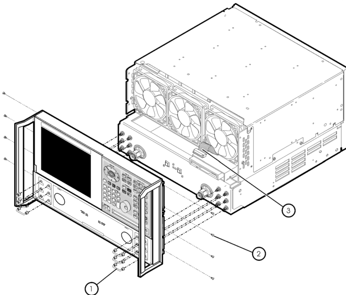
Figure 16 Front Panel Assembly Removal and Reinstallation (E8361A/C Only)
