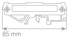
Side view (with casing)
