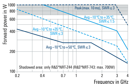
Maximum forward power of the R&S®NRT-Z43 and R&S®NRT-Z44 directional power sensors (for both directions)
