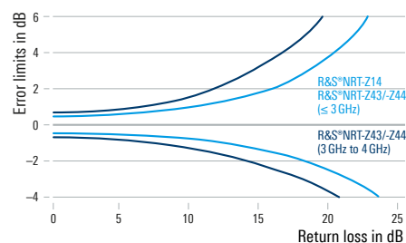
Measurement error limits (two standard deviations) for reflection measurements with the R&S®NRT-Z14/-Z43/-Z44 directional power sensors
