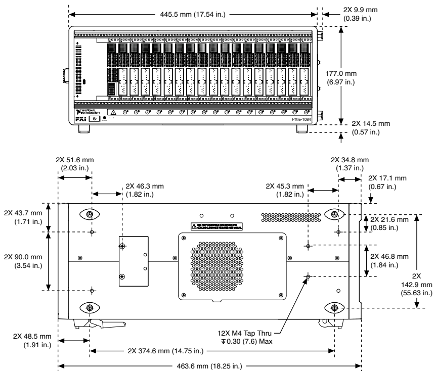
Figure 1. PXIe-1084 Chassis Dimensions (Bottom)
