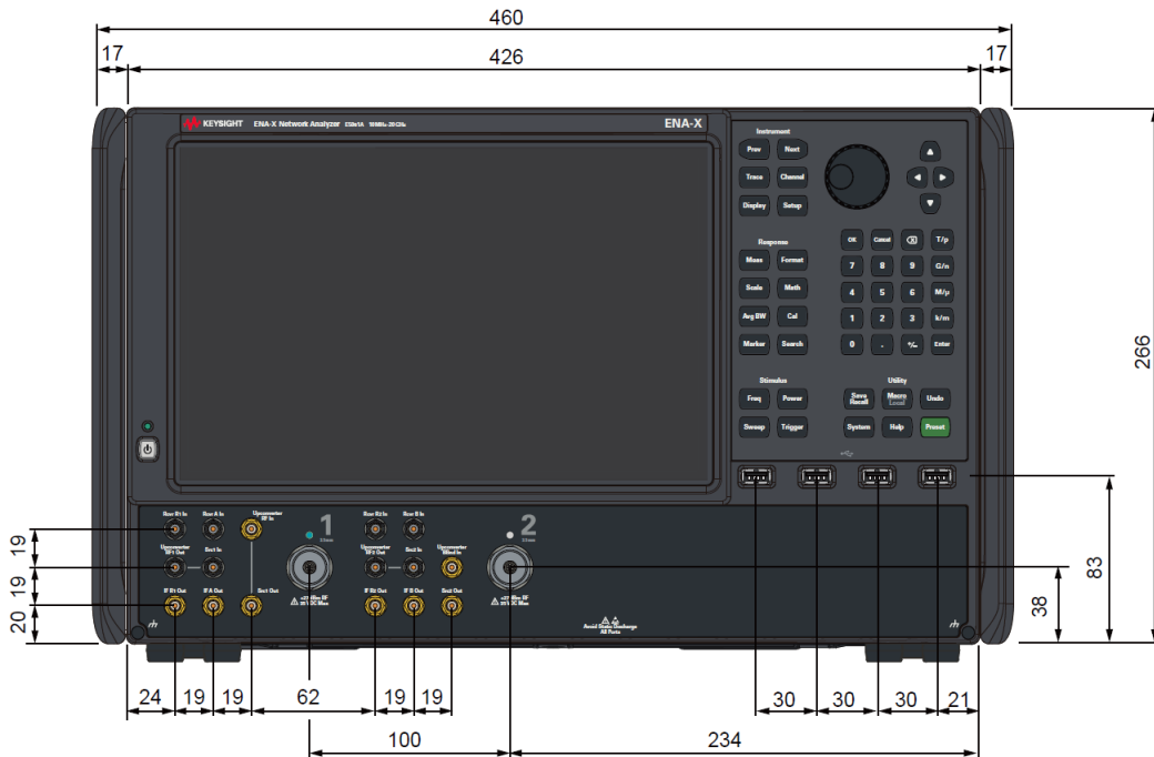
Dimensions (front view, E5081A with option 2K6, in millimeters)
