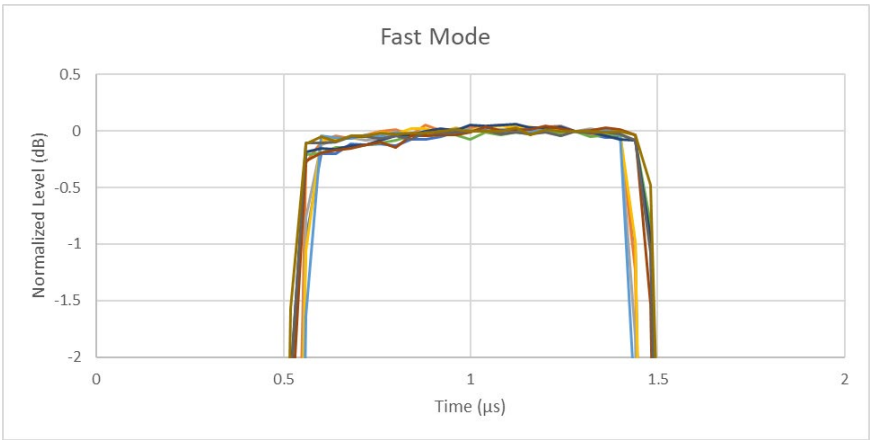
2. Measured with a 15 MHz IF bandwidth, averaging factor of 16 (Average Type = Point). With 1 μs pulse width setting. 0.5 μs/div. S960251B software is required. (Minimum pulse width with S960241B is 50 μs.)
