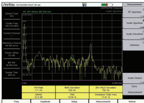
AM/FM/PM Analyzer
