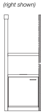
Hospitality Center (K/D) 4640D23CXLA / RA GR-310 32 1/2 x 22 1/2 x 90
