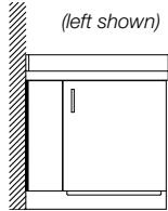
Hospitality Center 4640D23PXXLA / RA GR-302L / GR-302R 35 x 22 x 38
