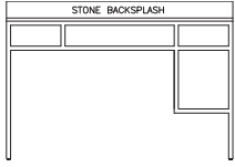
Vanity (left shown) 4640D21DXXLA / RA GR-326 54 x 24 x 38
