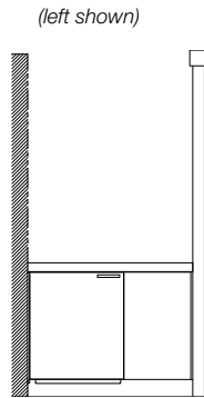
ADA Hospitality Center 4640D23UXXLA / RA GR-307 45 1/2 x 22 1/2 x 90
