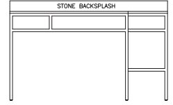
Vanity (left shown) 4640D21EXLA / RA GR-328 60 x 22 x 38
