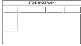
Vanity (left shown) 4640D21AXXLA / RA GR-313 68 x 24 x 38
