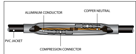
USEB-90 Splice Kit
