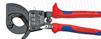
Ratchet Cable Cutter Black lacquered tool, handles with multi-component grips. Good for cutting copper and aluminium single conductors as well as multiple stranded cables. Little handforce required due to very high transmission ratio.
