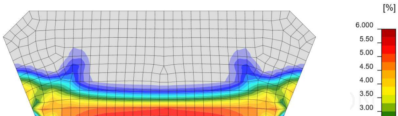
a) Strain check in CBFEM [%]
