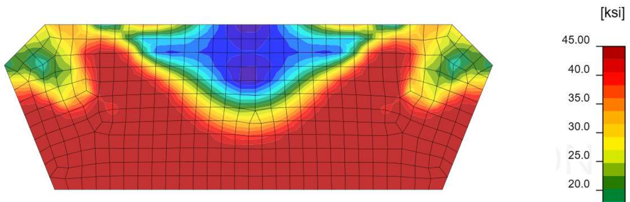
c) Check of von-Mises stresses in CBFEM for gusset plate above beam [ksi]
