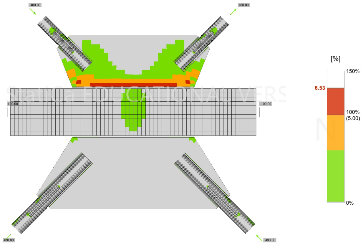
a) Strain check in CBFEM [%]
