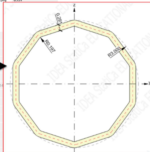
Figure 4 - The brace members as equivalent cold-formed sections in IDEA StatiCa
