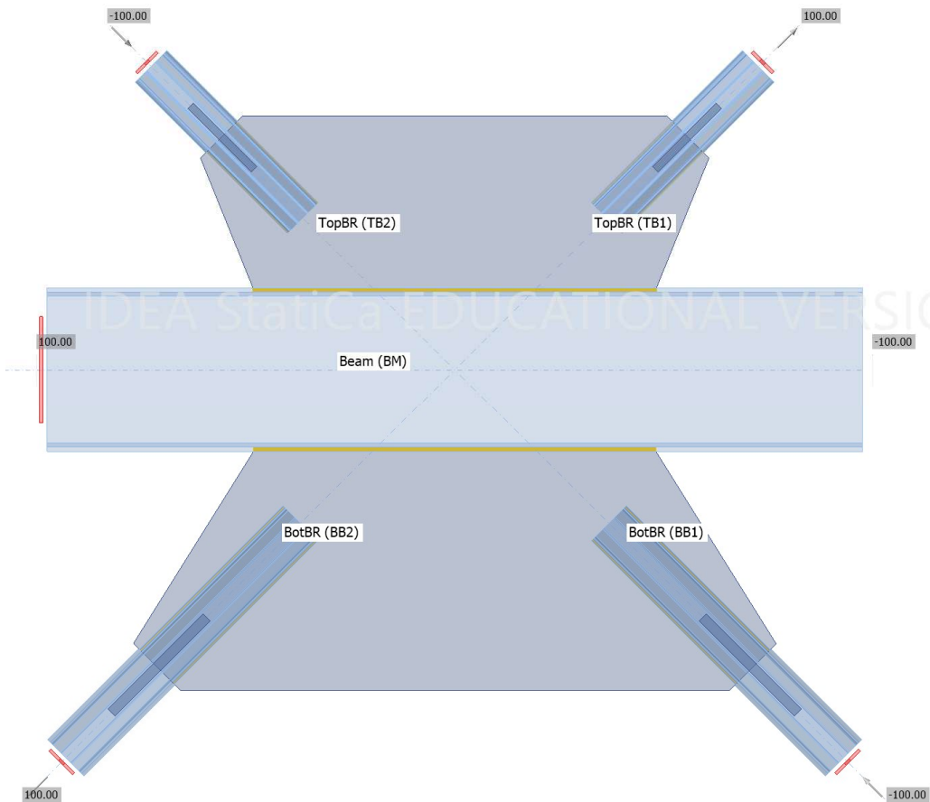
b) Transparent view of Base Model in CBFEM
