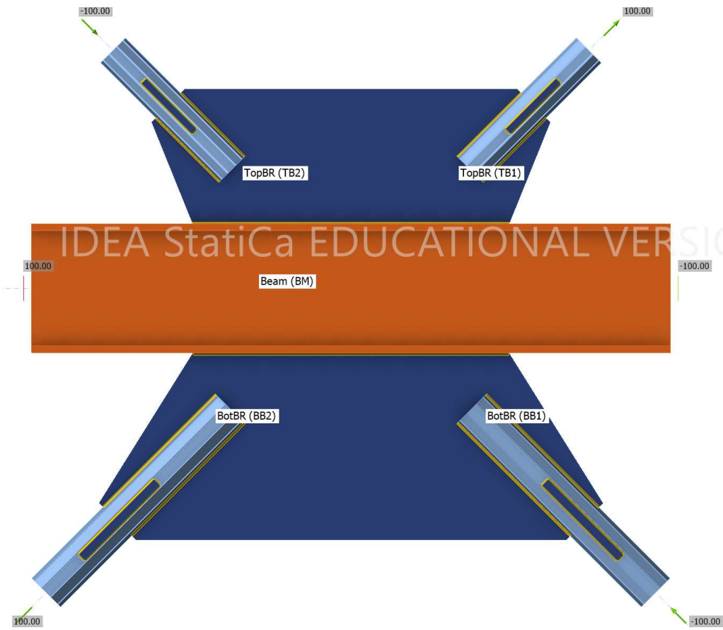
a) Solid view of Base Model in CBFEM
