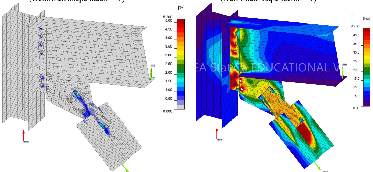
c) Plastic strains for P_{\text{tension}} = 105 kips (Deformed shape factor = 1)
