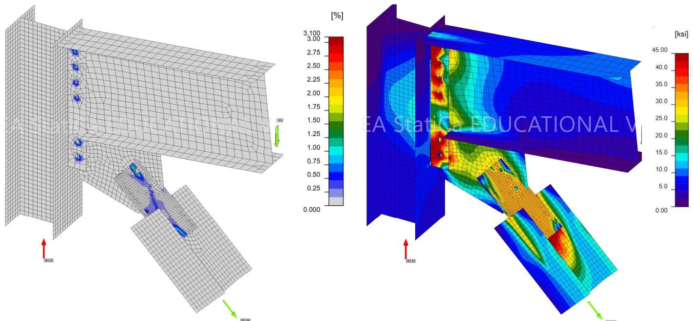
b) Plastic strains for P_{\text{tension}} = 101 kips (Deformed shape factor = 1)
