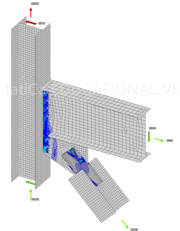
b) Plastic strains - CBFEM
