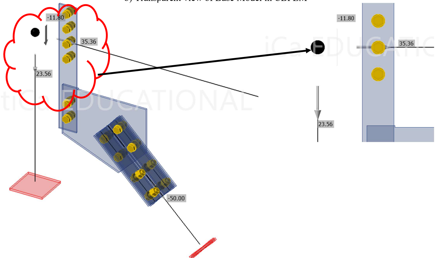
c) Wireframe view of Base Model in CBFEM
