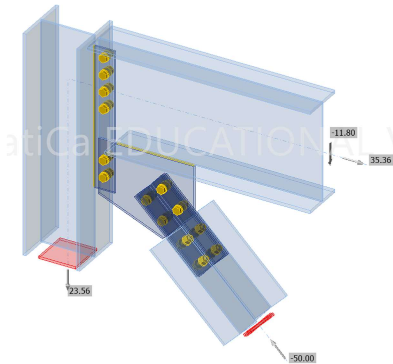
b) Transparent view of Base Model in CBFEM
