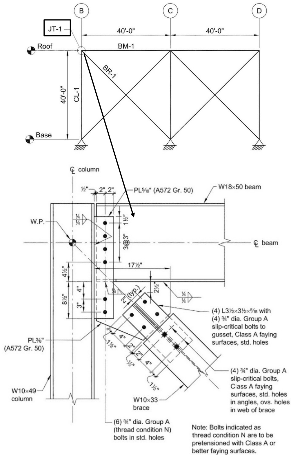
Figure 3 - Elevation of steel building and considered corner connection details (AISC 341, 2016)
