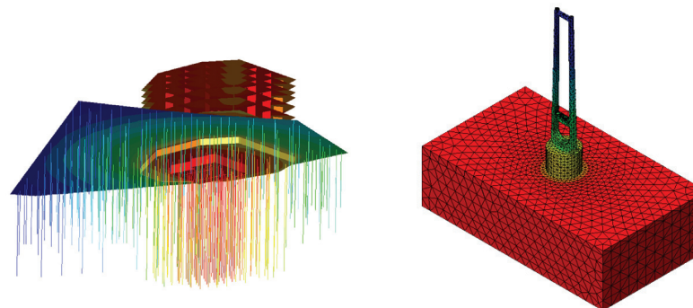
Deep Piled Raft Foundation ▲
