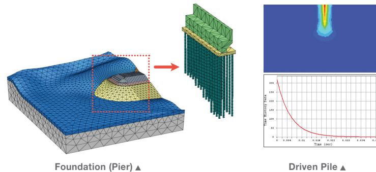
Foundation (Pier) ▲
