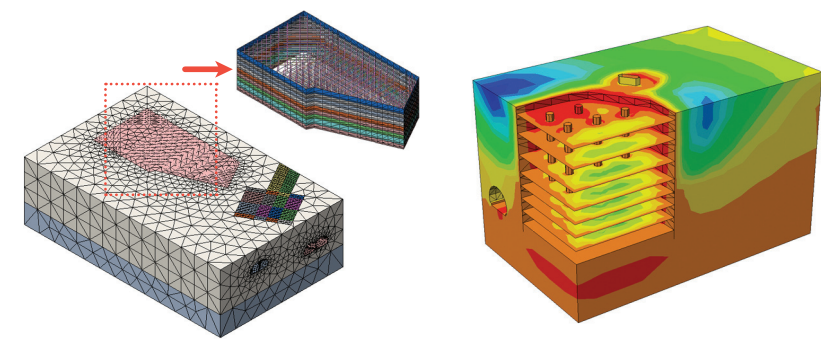
Ground shoring for excavation for a tall building foundation ▲
