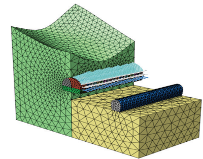
Steel pipe reinforced grouting (Pipe Roof) ▲
