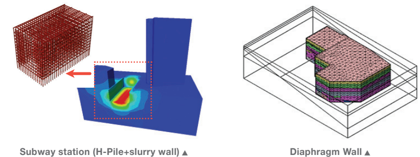
Subway station (H-Pile+slurry wall) ▲
