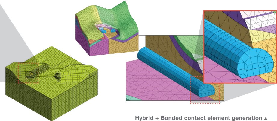
Hybrid + Bonded contact element generation ▲
