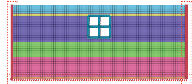
Dynamic analysis (soil structure interaction) boundary generation ▲
