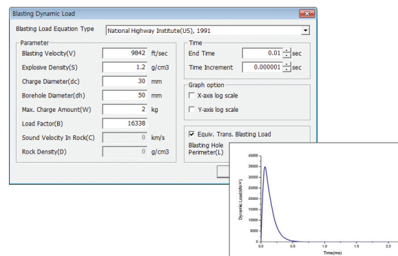
Dynamic blast load automatic generation ▲
