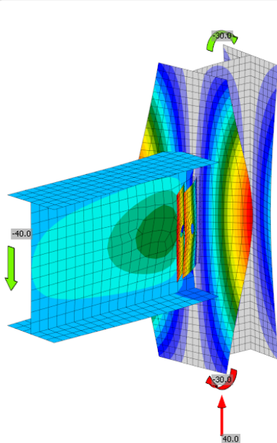
Local buckling of joint
